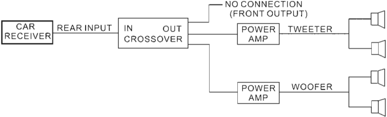
(B) 2-Channel Two-Way System (tweeter + woofer)
