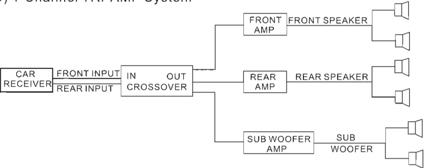
(C) 4-Channel TRI-AMP System
