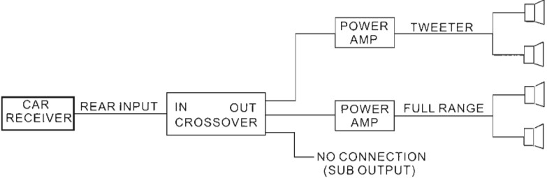
(A) 2-Channel Two-Way System (tweeter + full range)
